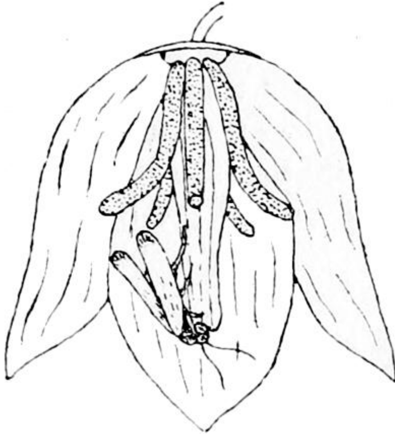
FIG. 14.—Yucca Flower and Moth.
