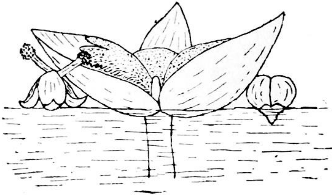
FIG. 8.—Flower of Valisneria .
