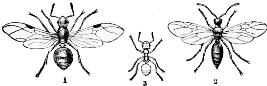
FIG. 24.—Wood ant. 1, Queen; 2, male; 3, worker (from Shipley).
