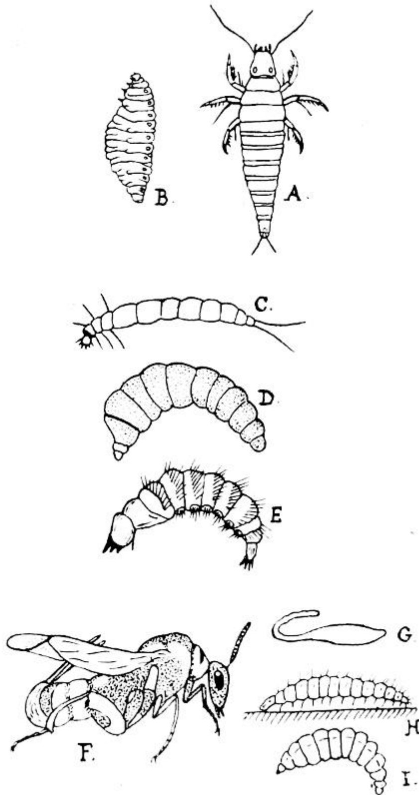
FIG. 13.—Insect Larvæ. A, B, of Sitaris ; C, D, E, of Argyromœba ; G, H, I, of Leucopsis ; F, imago of Leucopsis (after Fabre).
